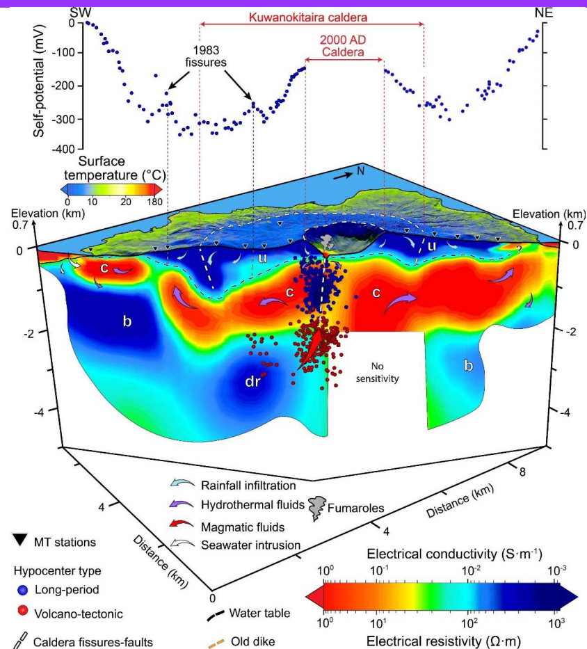
Hypocenters determined by JMA
